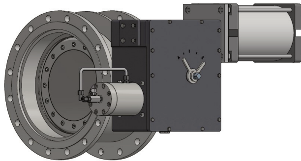
Figure 5-6: combined butterfly/check valve with a pneumatic actuator
