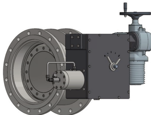
Figure 5-5: combined butterfly/check valve with an electric actuator
