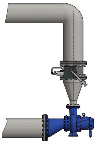
Figure 5-1: Position in the pipeline / 1
