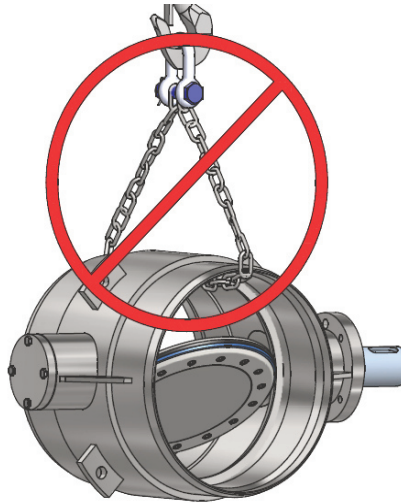
Figure 4-5: Attachment through the valve body
