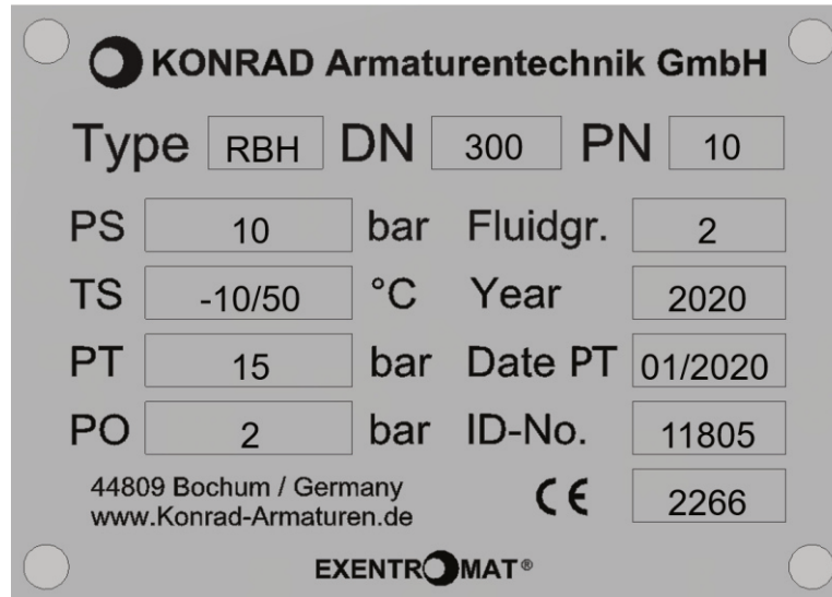
Figure 3-2: Nameplate
