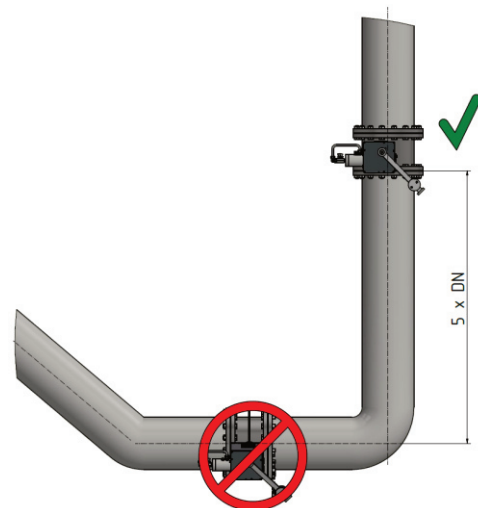
Figure 5-2: Position in the pipeline / 2
