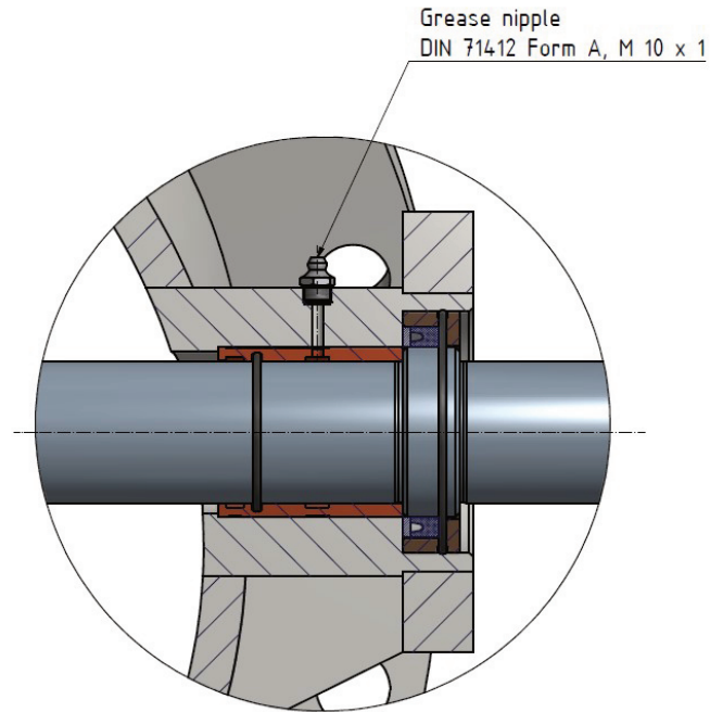
Figure 7-1: Grease block chamber
