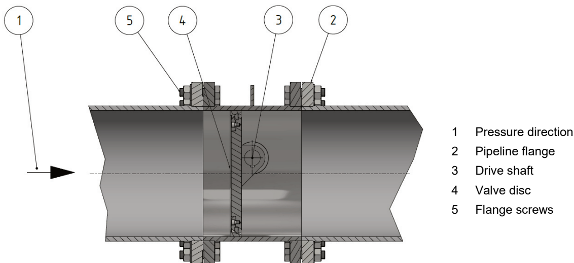
Figure 5-3: Check valve cross section
