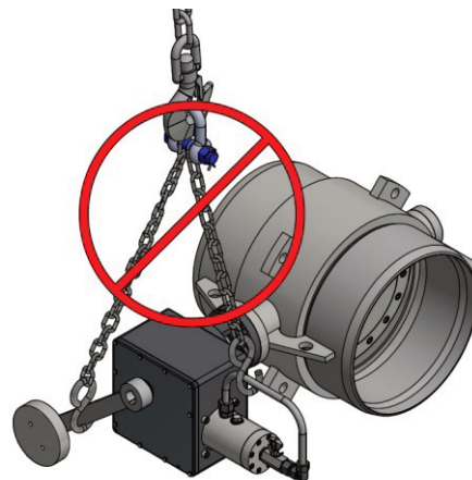
Figure 4-4: Attachment to the lever and pipe
