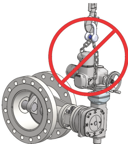
Figure 4-3: Attachment to the actuator
