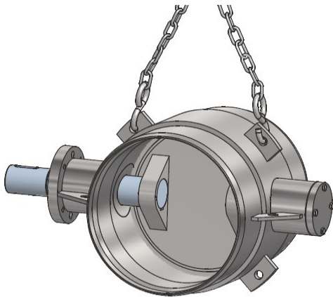
Figure 4-1: Attachment to the crane lugs
