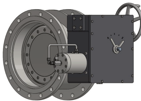
Figure 5-4: combined butterfly/check valve with a manual actuator using a handwheel
