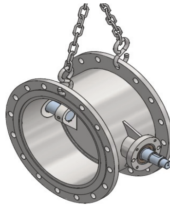
Figure 4-2: Attachment to the flange holes
