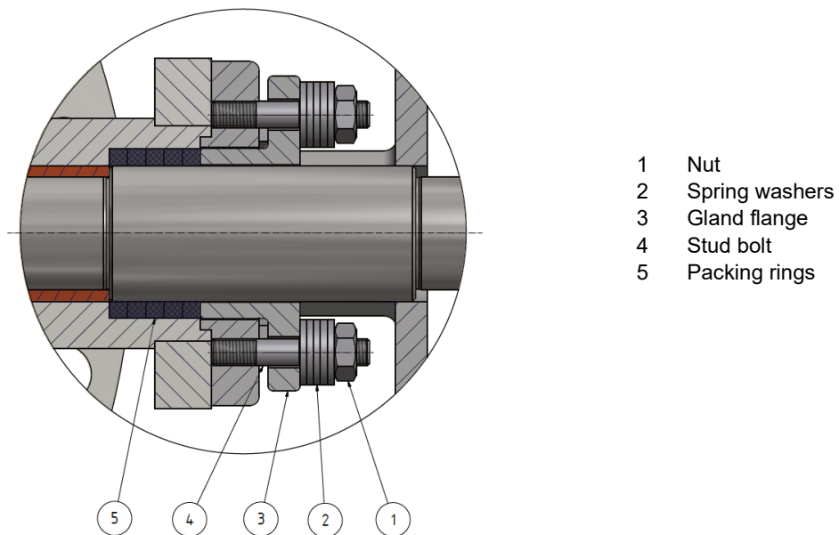
Figure 7-2: Gland
