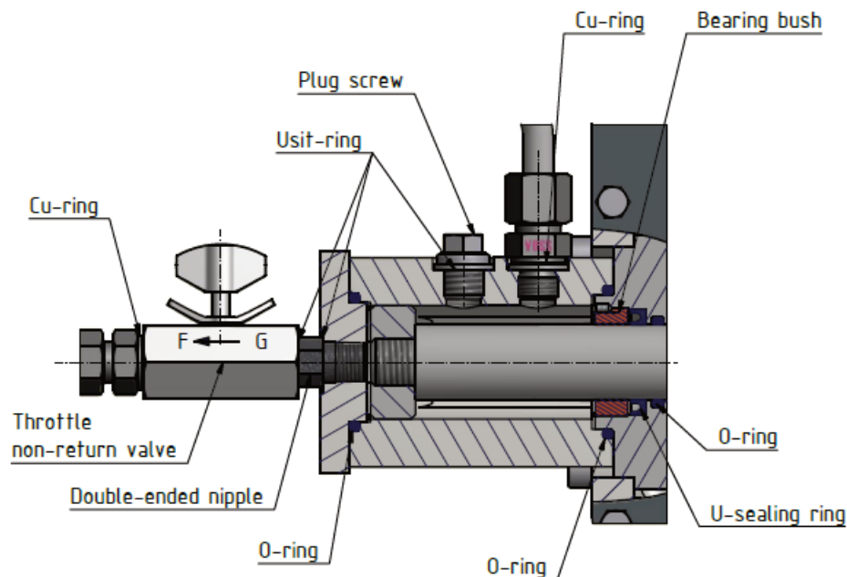
Figure 7-3: Hydraulic brake cylinder
