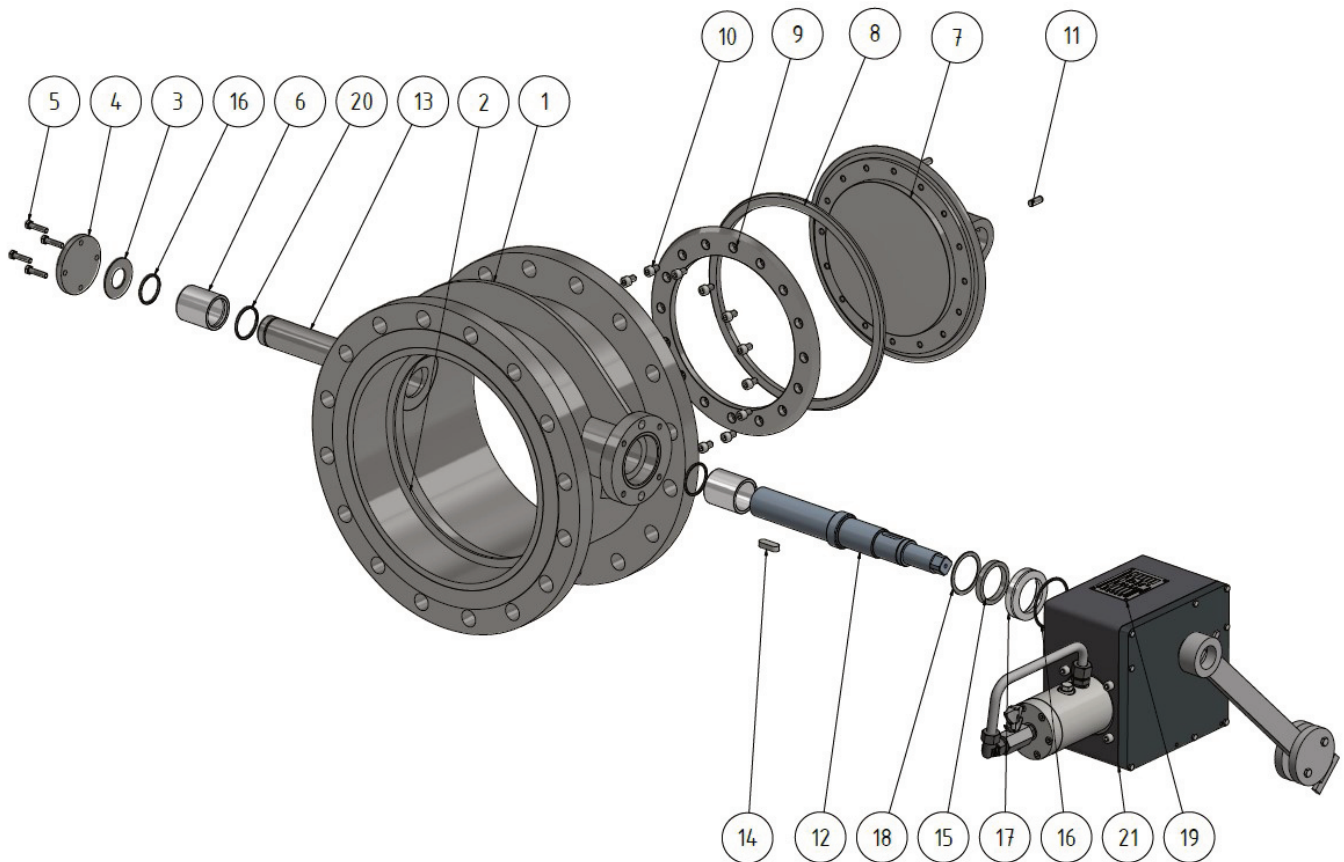
Figure 3-1: Example illustration of a check valve, type RBH
