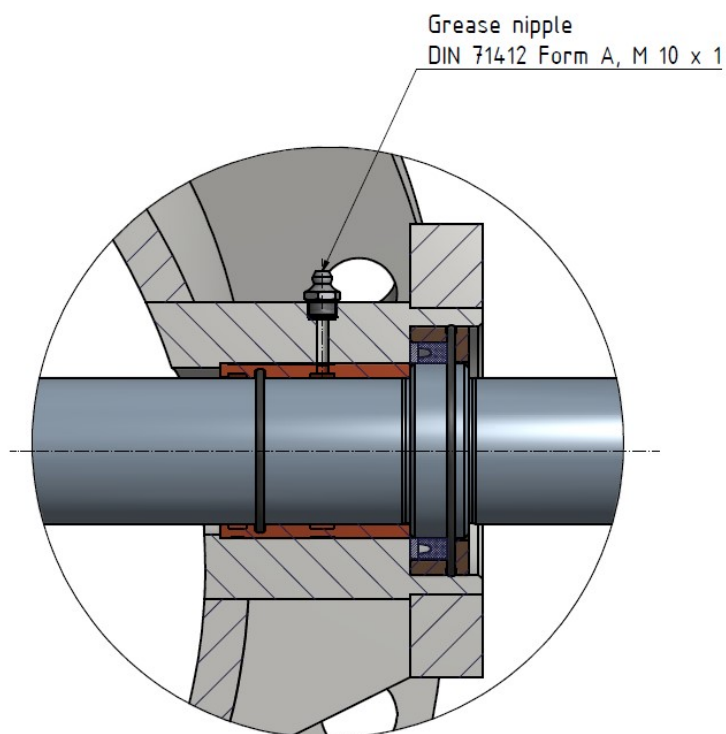
Figure 7-1: Grease block chamber
