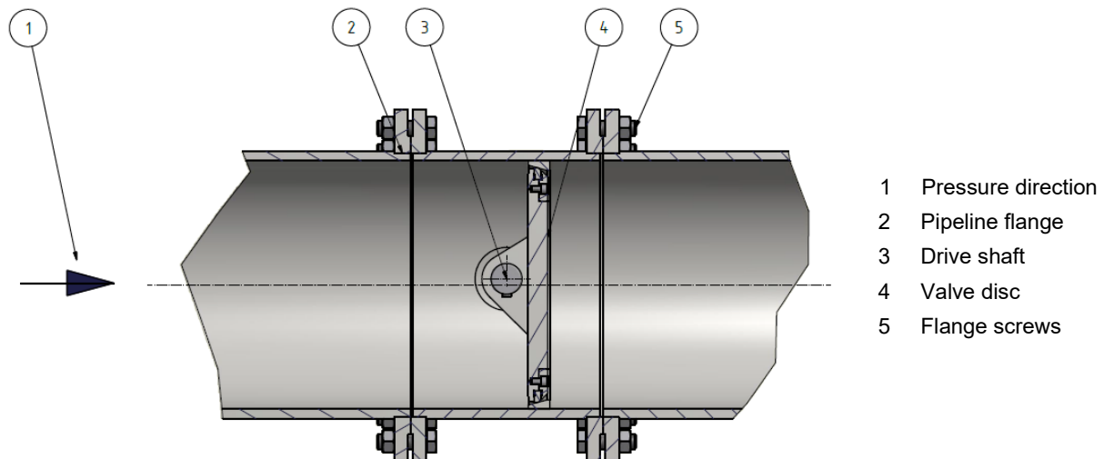
Figure 5-3: Butterfly valve cross section
