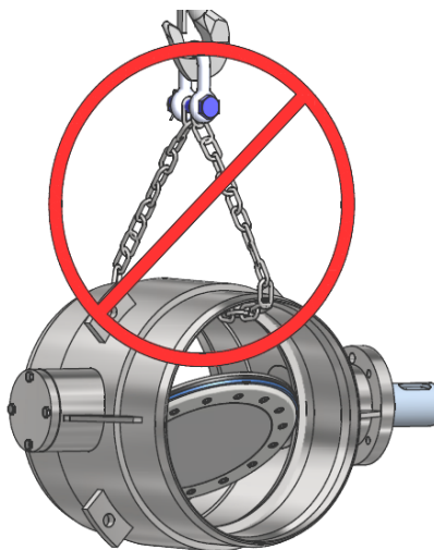
Figure 4-4: Attachment through the valve body
