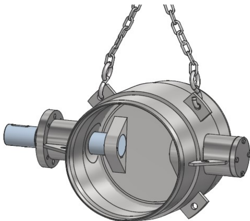
Figure 4-1: Attachment to the crane lugs
