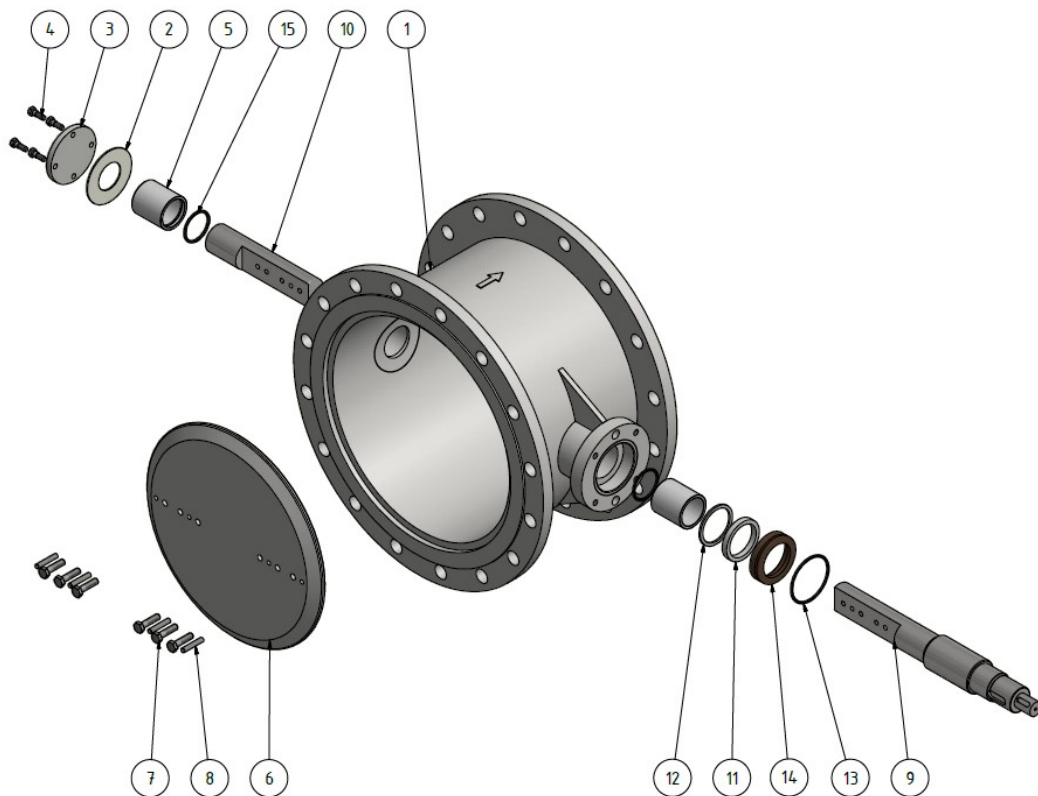
Figure 3-2: Example illustration of a throttle valve
