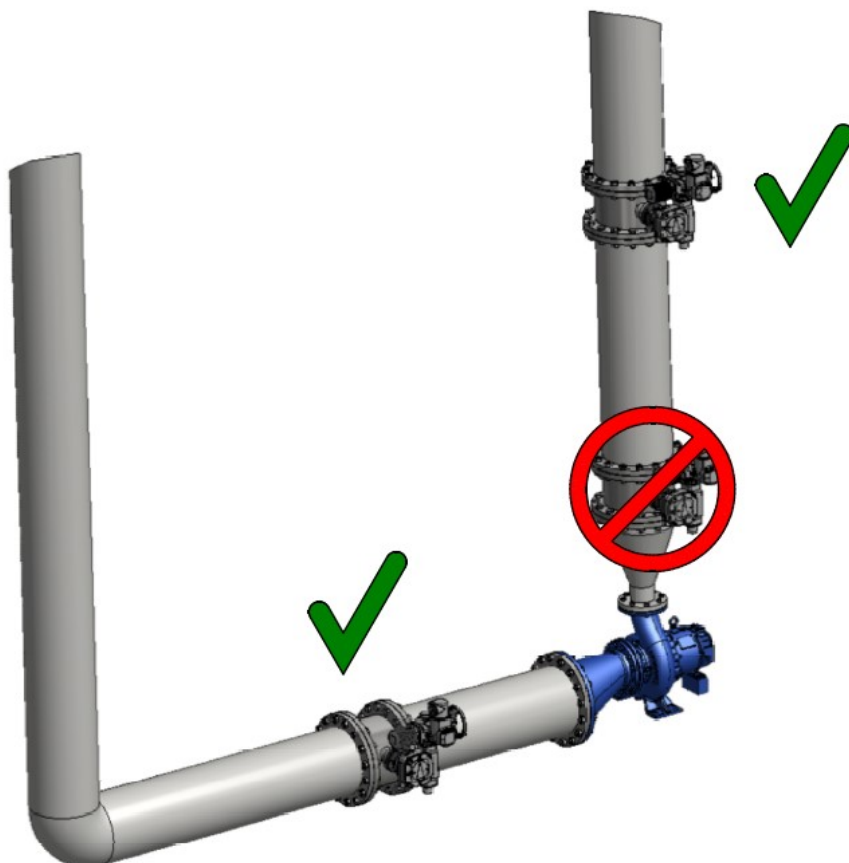
Figure 5-1: Position in the pipeline / 1
