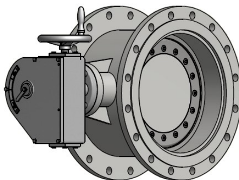
Figure 5-4: Butterfly valve with manual actuator using a handwheel
