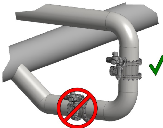
Figure 5-2: Position in the pipeline / 2
