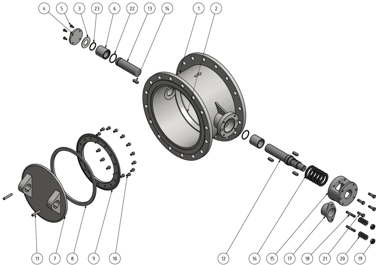
Figure 3-1: Example illustration of a butterfly valve
